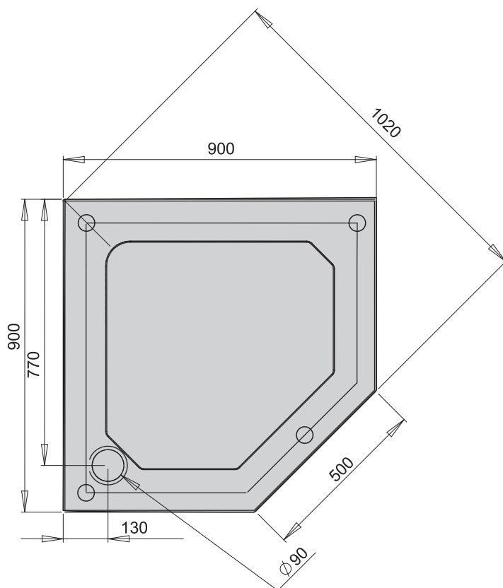
CLASSIC PPV44X
