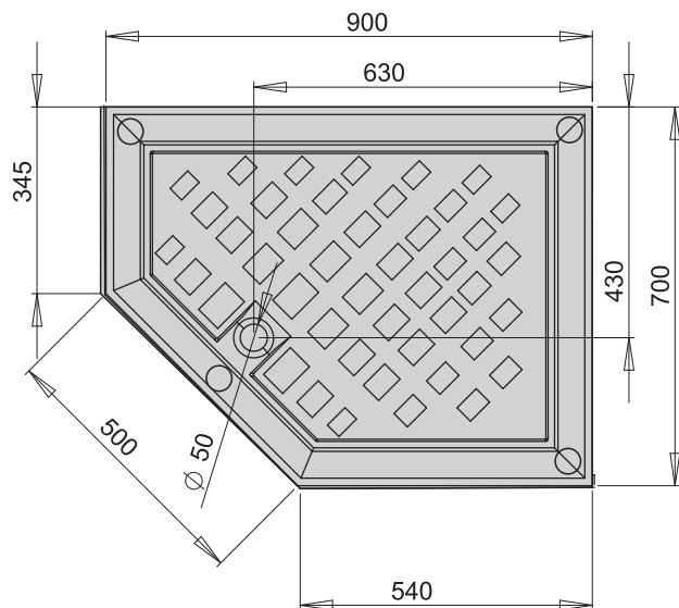
CLASSIC PPV24X
