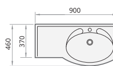
DELTA 900/L (IDE900/L/xx)
